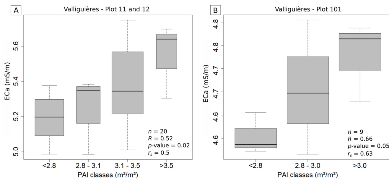
Figure 5. Boxplot of apparent electrical conductivity (ECa) from EM31 survey per classes of plant area index (PAI) classes at Valliguières: (A) plots 11 and 12 which both have 600 stems/ha and, (B) plots 101, which both have 400 stems/ha. n is the number of value, R is Pearson correlation, p -value is calculated on Pearson correlation, r_s is the Spearman correlation.
