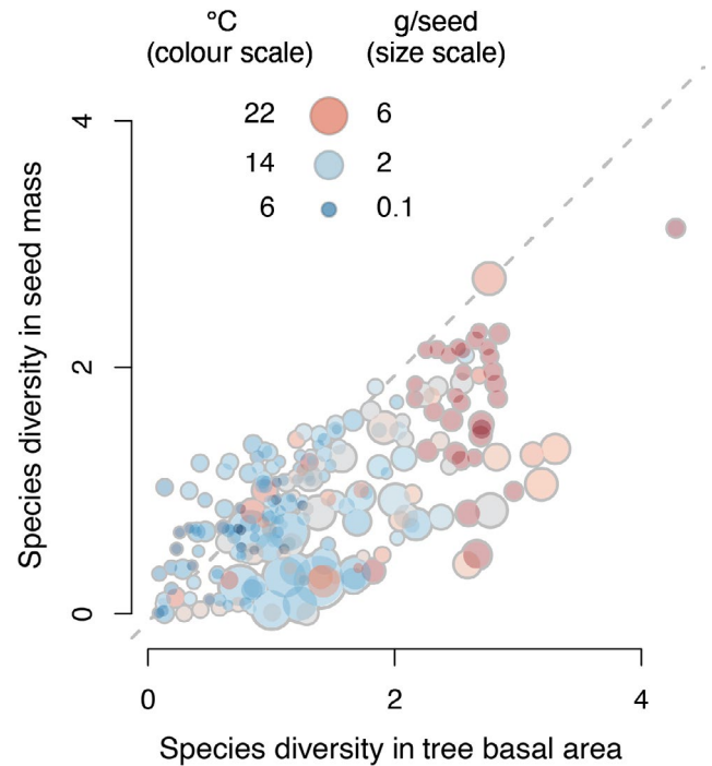
FIGURE 6 Species diversity in seeds (vertical axis) is lower than expected from species diversity in trees (horizontal axis). In both cases, diversity is evaluated from the Shannon index, -\sum p_s \log p_s , where p_s is the fraction of species s in basal area (trees) and CSP (seed mass). Each point represents an inventory plot. Except at low tree diversity, points lie almost entirely below the 1:1 line (dashed). The legend at top left shows mean annual temperature (symbol colour) and mass of the average seed (symbol size)
